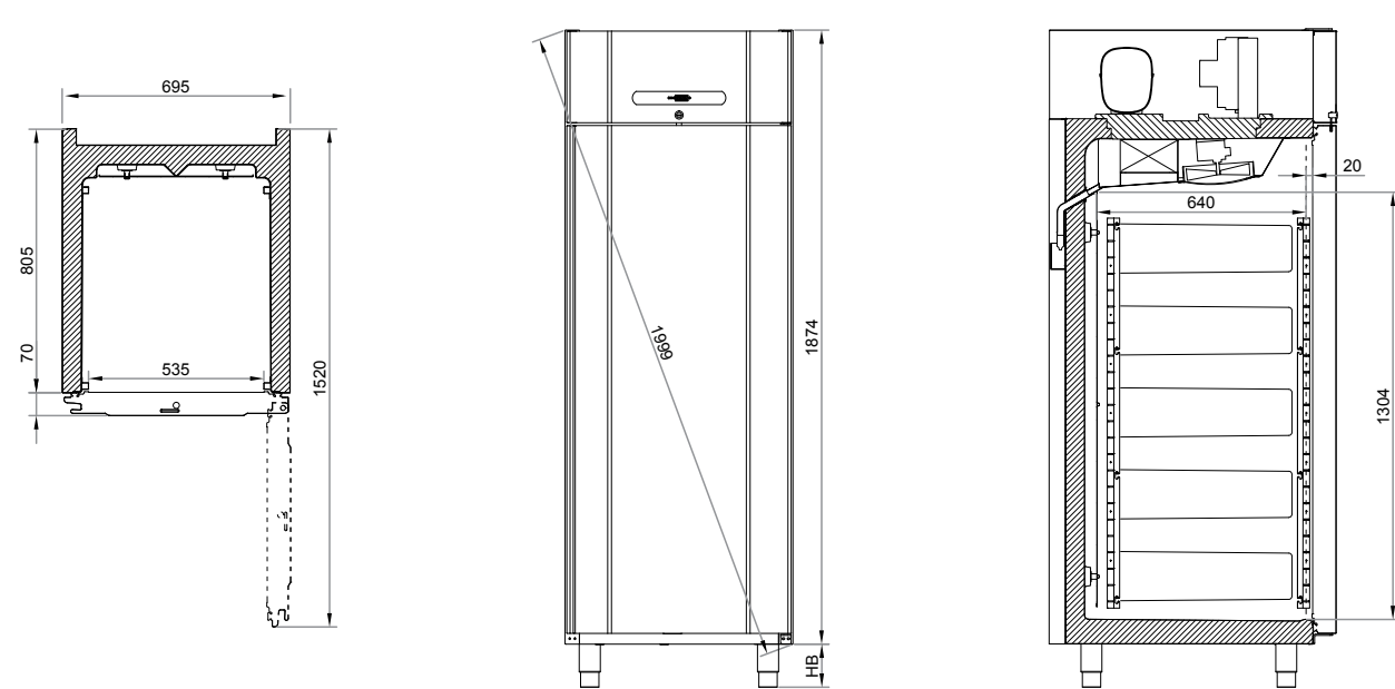
BioCompact II 410
