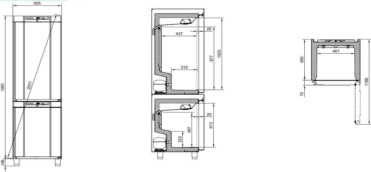
BioCompact II 210/210 / 310/210
