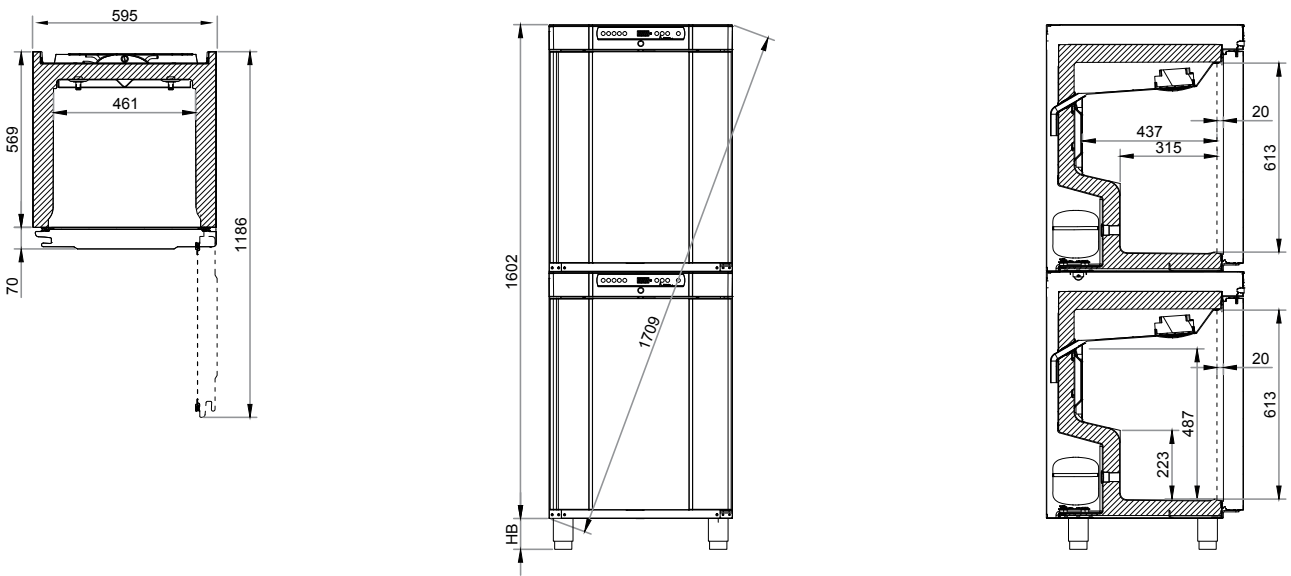
BioCompact II 210/210
